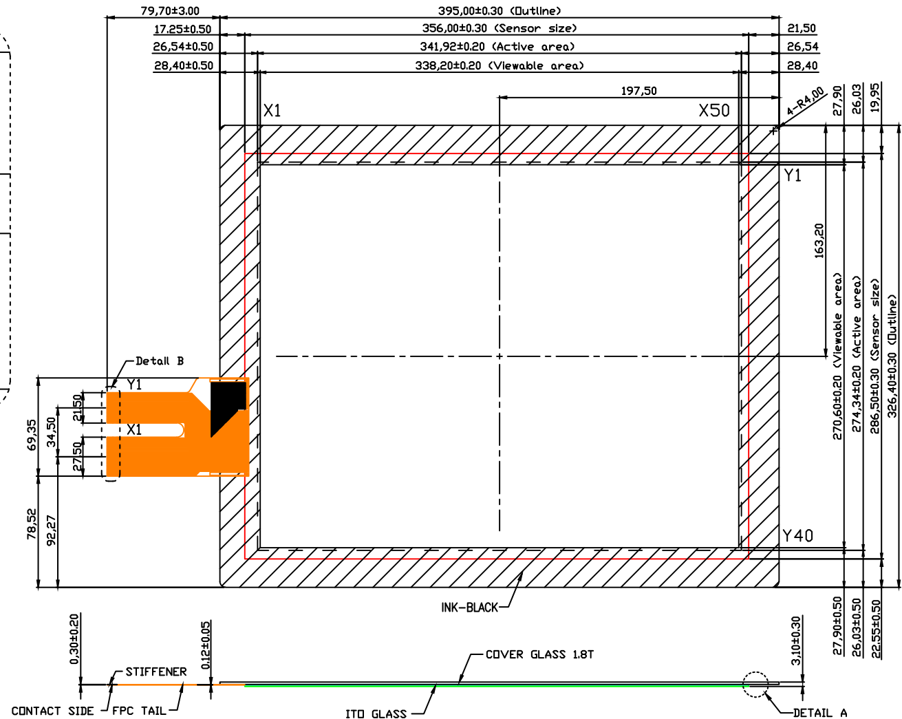
DETAIL B
